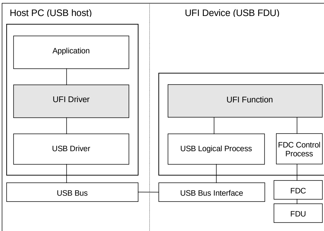
Figure 1 - Host/UFI Device Conceptual View
